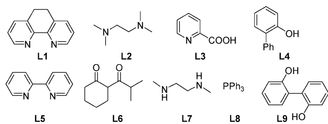
Figure 1. Ligands tested for the synthesis of 4a (see Table 1).
